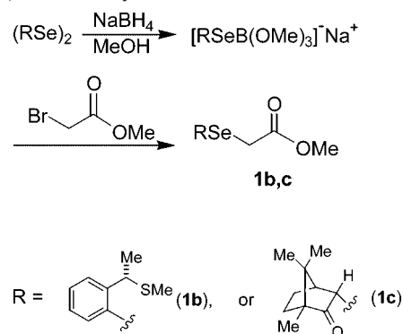
Scheme 2. Synthesis of the methyl [(2-[(1 S )-1-(methylthio)ethyl]phenyl}seleno]acetate ( 1b ) and the methyl ( R )-camphorselenoacetate 1c
