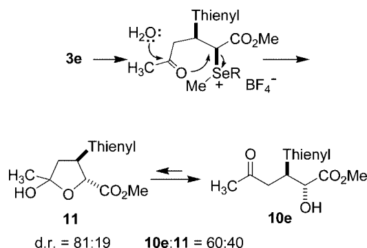
Scheme 6. Reaction of the \delta -oxo- \alpha -seleno ester 3e with trimethyloxonium tetrafluoroborate
