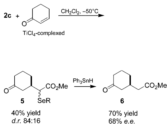
Scheme 3. Nucleophilic addition of the titanium enolate 2c to cyclohex-2-en-1-one
