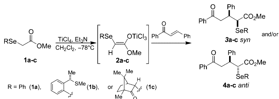
Scheme 1. Reactions of chalcone with the methyl selenoacetates 1a–1c
