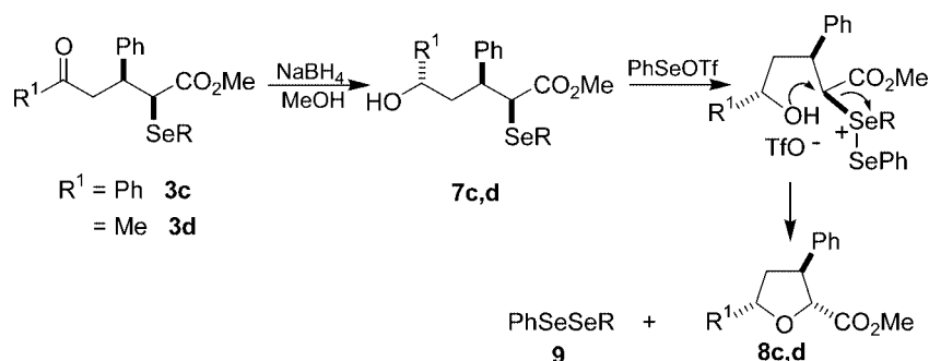
Scheme 4. Synthesis of enantiomerically pure trisubstituted tetrahydrofurans 8c,d
