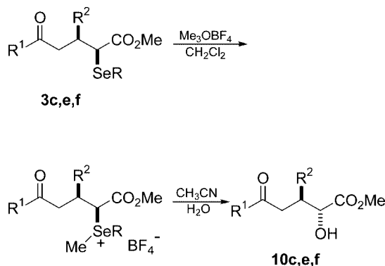
Scheme 5. Synthesis of \alpha -hydroxy esters from \alpha -seleno esters
